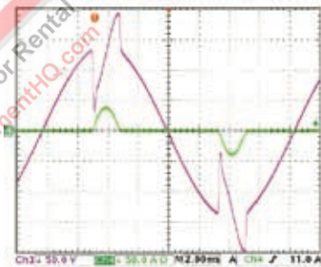
Figure 9: With ABA
