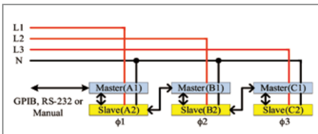
Figure 11: Parallel/3-Phase Y connection
